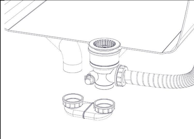
U Pipe 1
