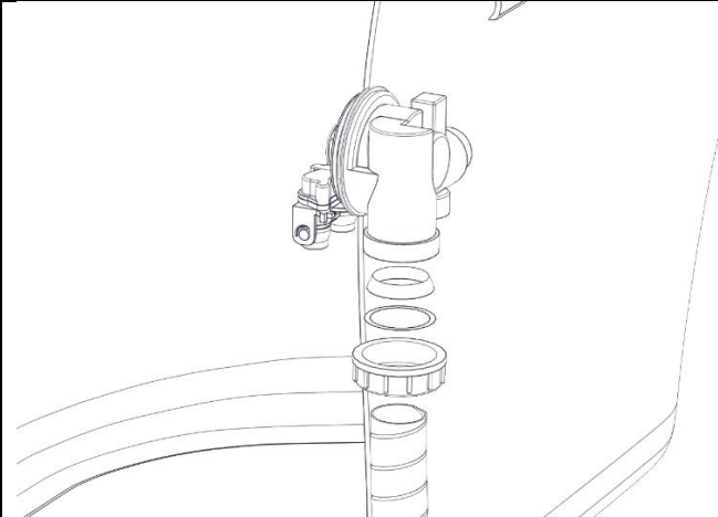
Overflow Pipe 1
