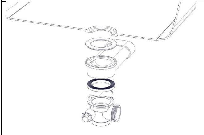
Drain Assembly 1
