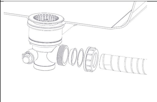
Drain Pipe 1
